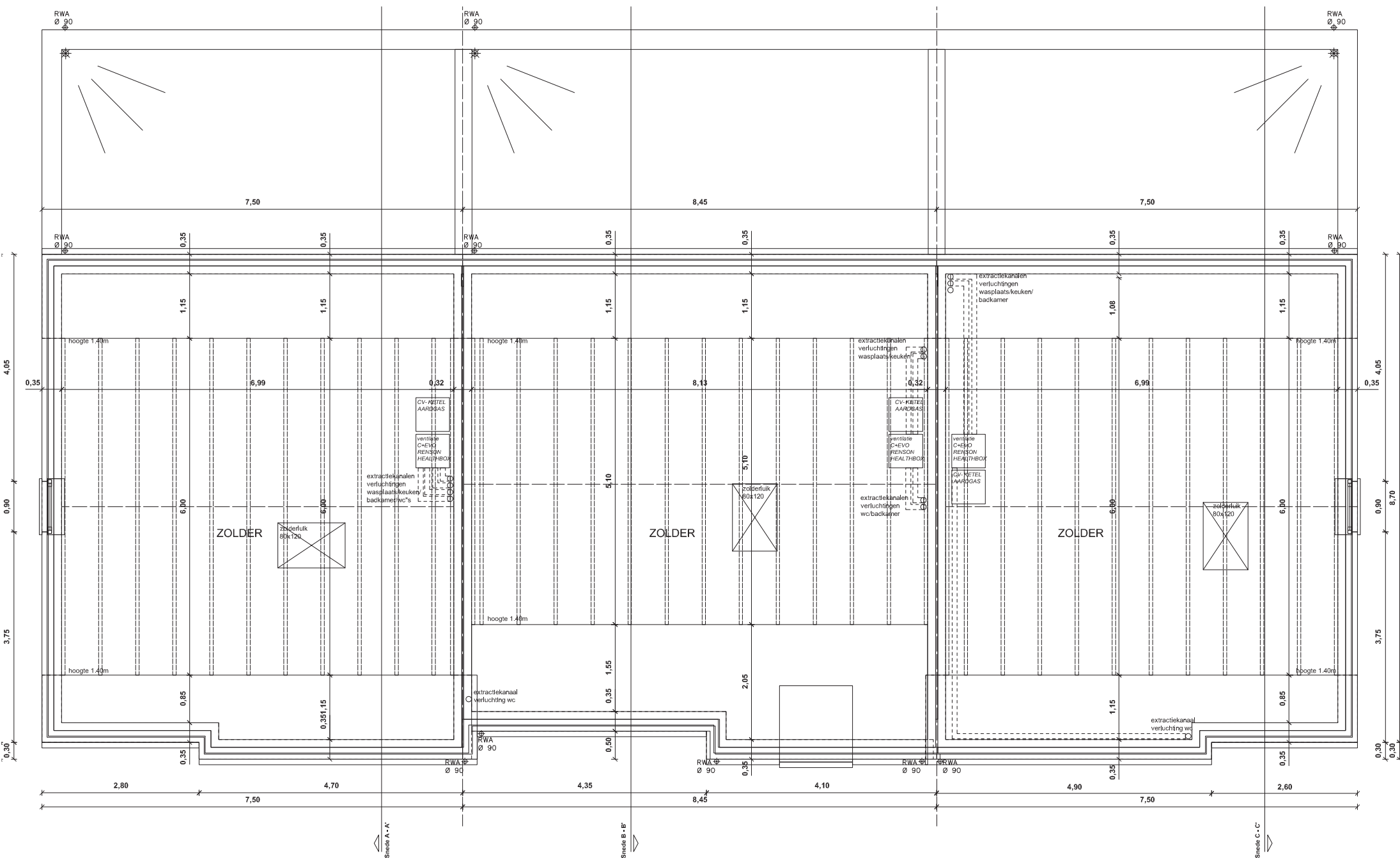
ZOLDERPLAN schaal 1/50
